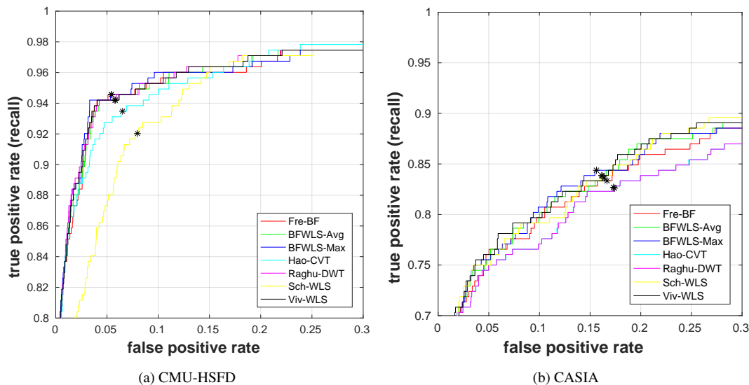
Figure 5: The ROC curves for the CMU-HSFD and CASIA datasets using DSIFT + Cosine Similarity method for verification tasks. * denotes the EER when the false accept rate is equal to the false reject rate. Best viewed in color.
